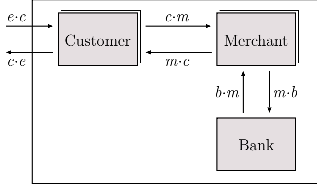
Figure 4: NetBill architecture
