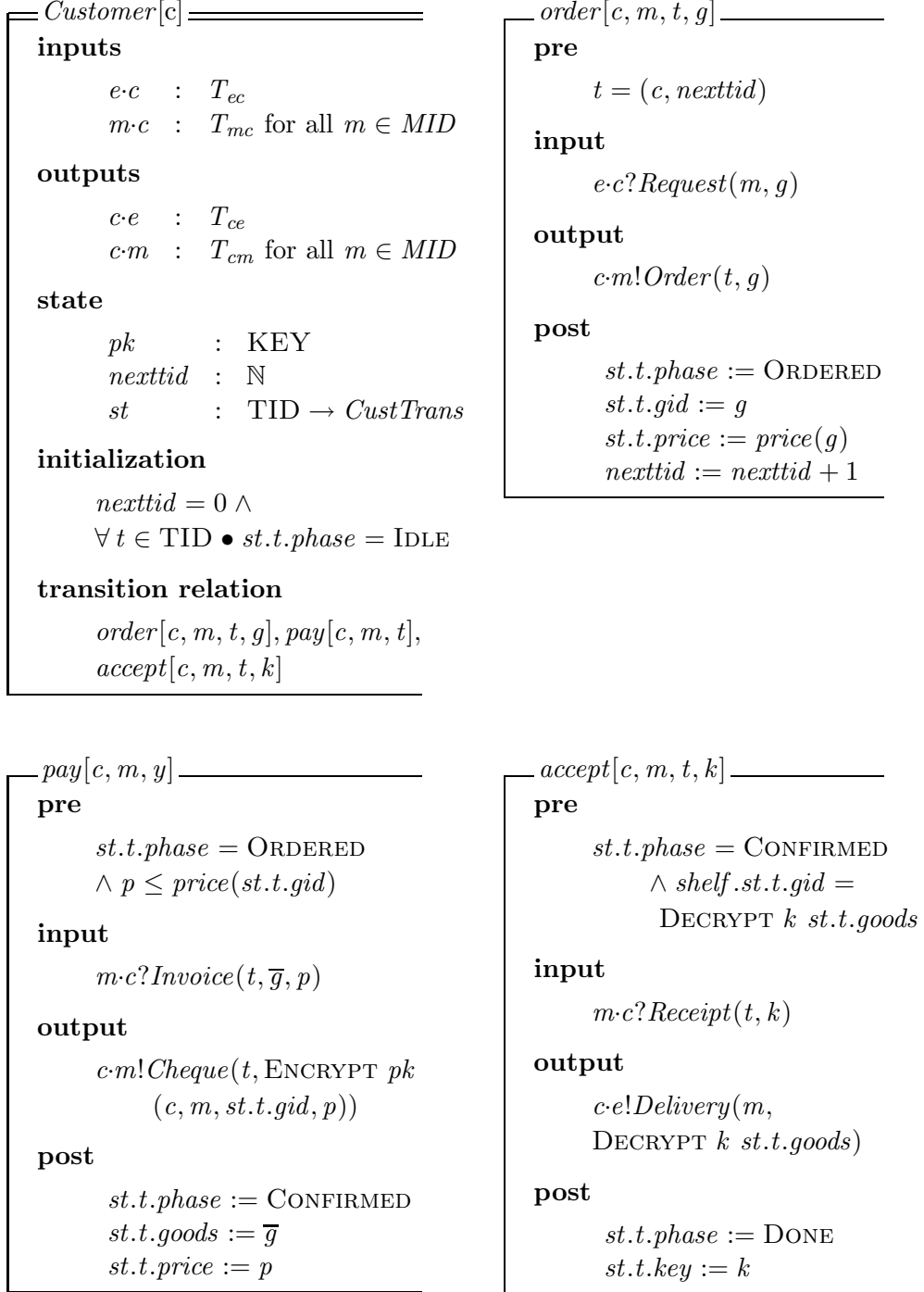
Figure 5: Customer Specification
