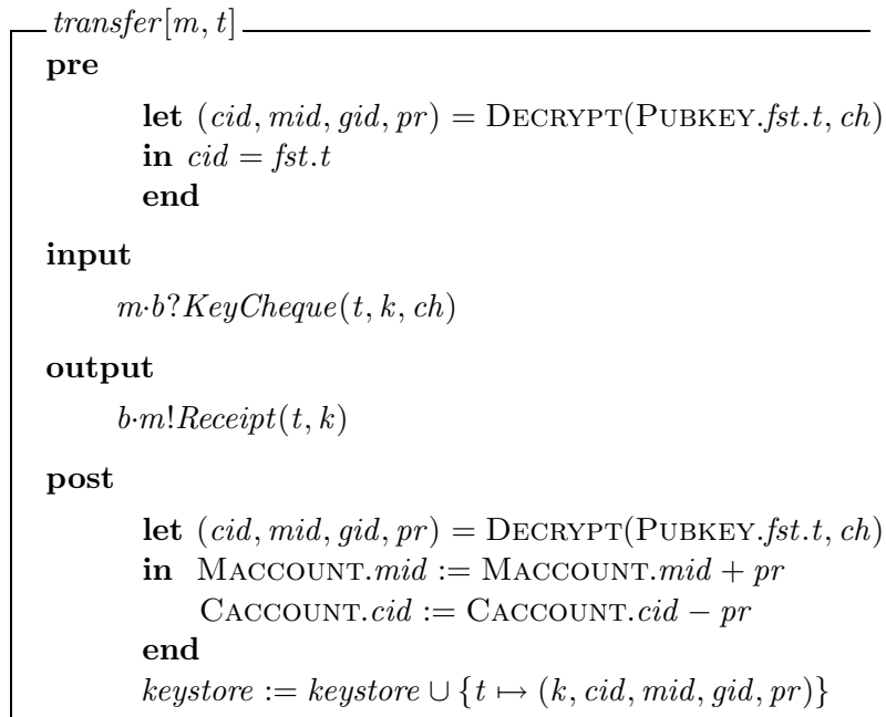
Figure 7: Bank Specification
