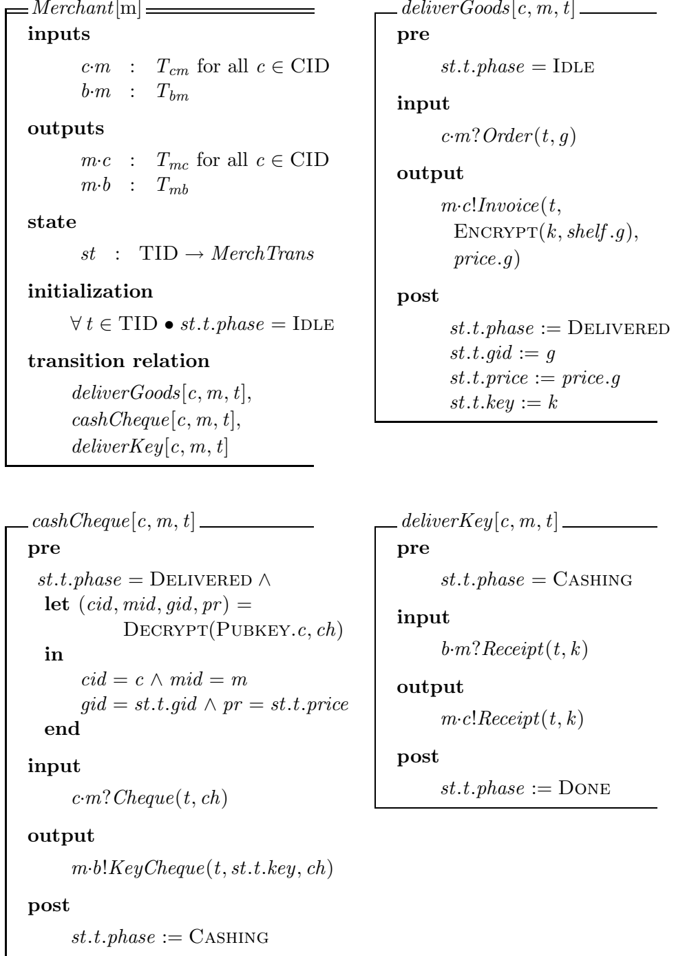
Figure 6: Merchant Specification
