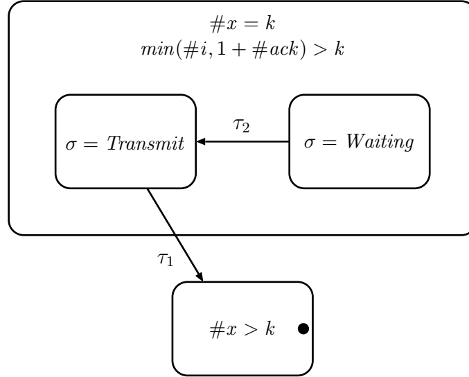
Figure 16: Leadsto Diagram for the Sender
