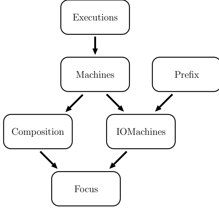
Figure 8: Theory Graph
