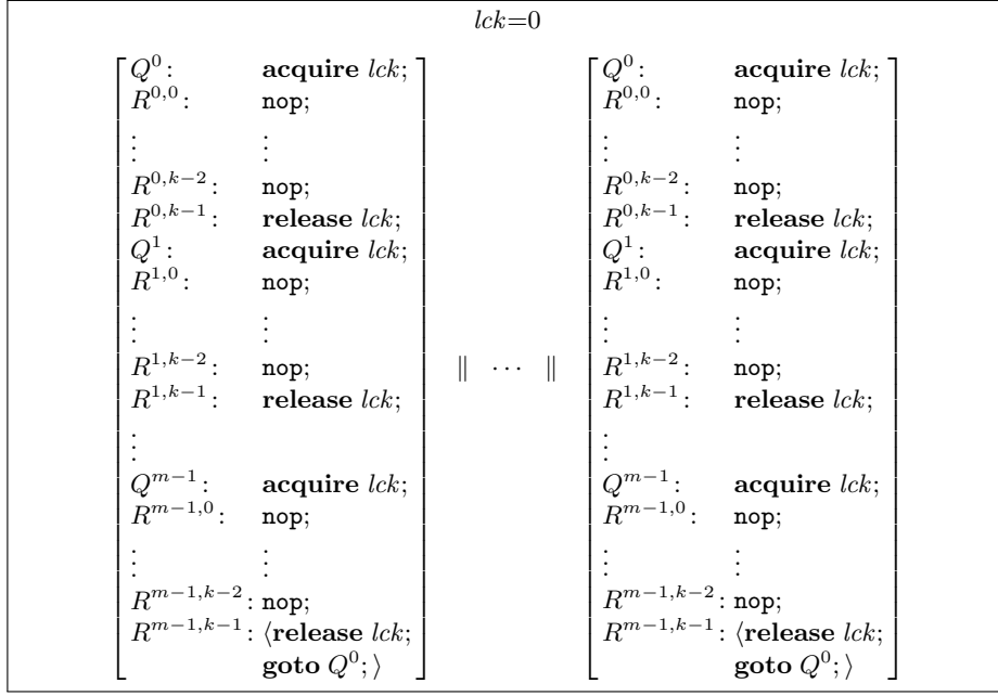
Fig. 4: A parameterized program consisting of n concurrent threads with m critical sections per thread such that each critical section has k control locations.
