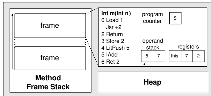
Fig. 1. The JVM.
