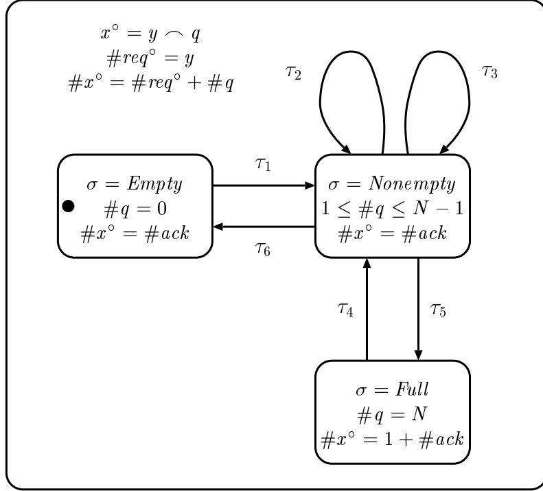
Figure 15: Queue Invariance Diagram
