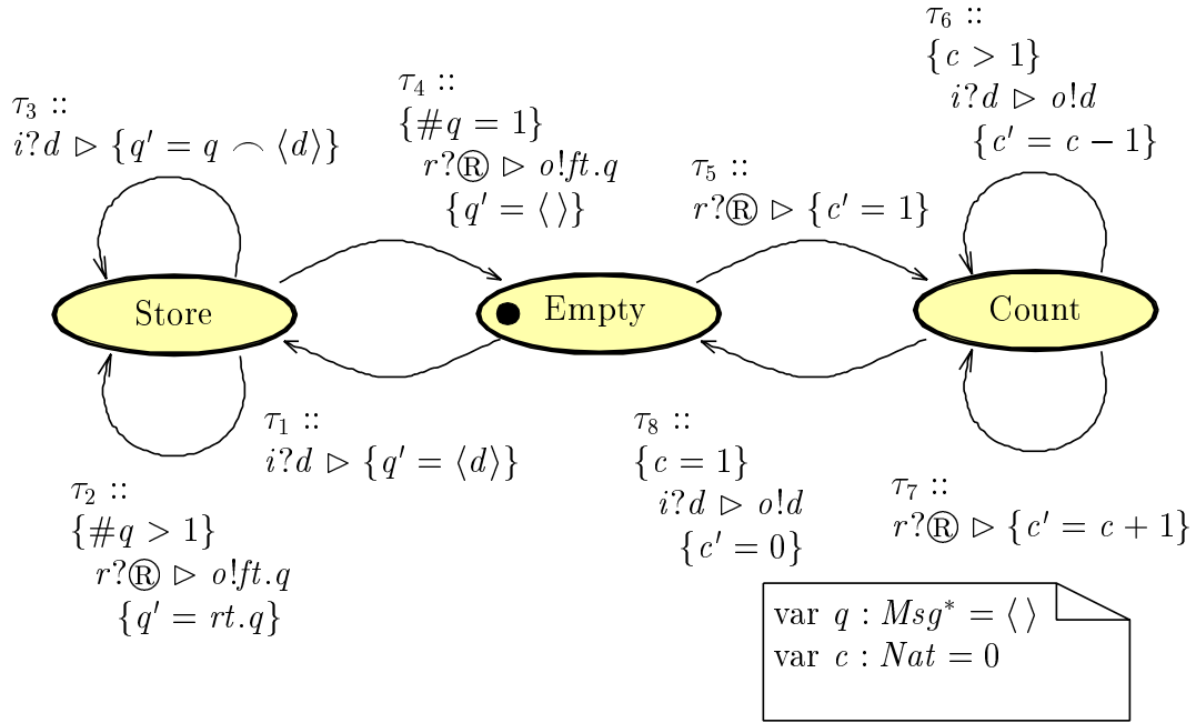
Figure 2: STD for the Buffer
