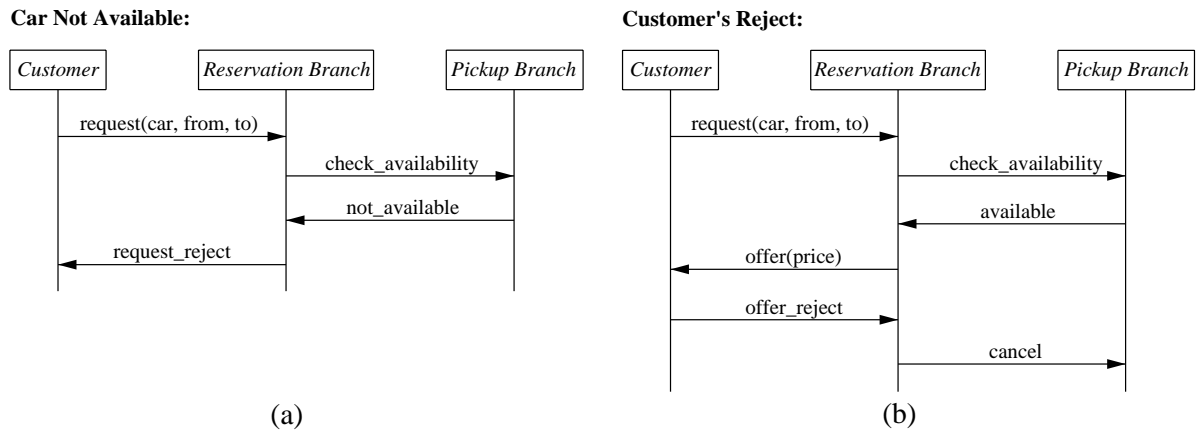
Figure 3: Exemplary Descriptions of an Unsuccessful Car Reservation
