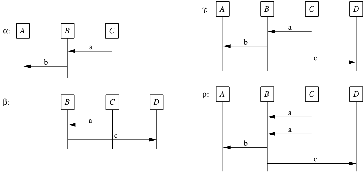
Figure 5: Parallel Composition of EETs: Two Possible Interpretations
